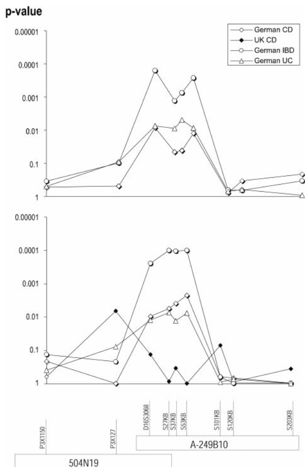
Fig. 2. Association analysis (transmission distortion as calculated by TRANSMIT ) of markers in the vicinity of the association signal in the vicinity of D16S3068. (Upper) The unstratified analysis of the German part of the extended cohort (no significant results were obtained in the United Kingdom part of the cohort, which have thus been omitted for clarity). (Lower) The results of the analysis of the NOD2 -stratified genotypes. The key of phenotypes and populations is given in Upper. The marker names and the corresponding physical map using the local BAC clones are shown below the association graphs.
